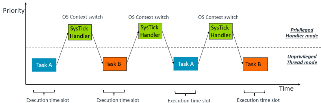
Fig. 1. Preemptive Context Switcher
