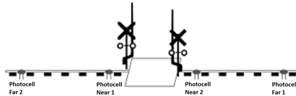
Fig. 5. Crossing Gate Image
