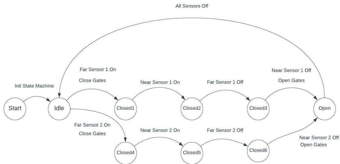
Fig. 6. Gate Control State Machine
